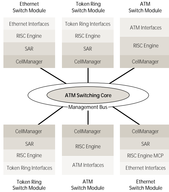
Figure 1 | Parallel LAN and ATM Switching with the Centillion 100 Architecture
